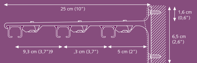
Aluminium Wall bracket triple
